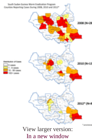
Figure 2. SSGWEP: counties reporting cases during 2008, 2010, and 2012.
