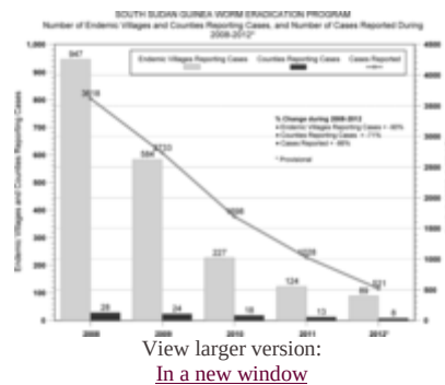
Figure 3. SSGWEP: the number of endemic villages and counties reporting cases and the number of cases reported during 2008–2012.
